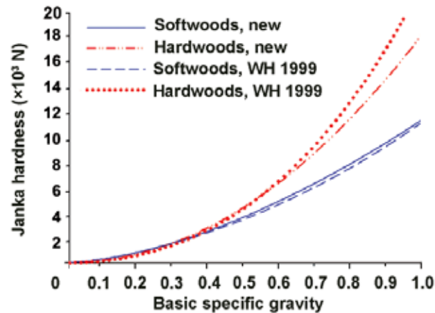
Figure 5—Comparison of our regression equations for hardness at 12% MC (new) with those given in the 1999 edition of the Wood Handbook after adjustment to G_g (FPL 1999).
